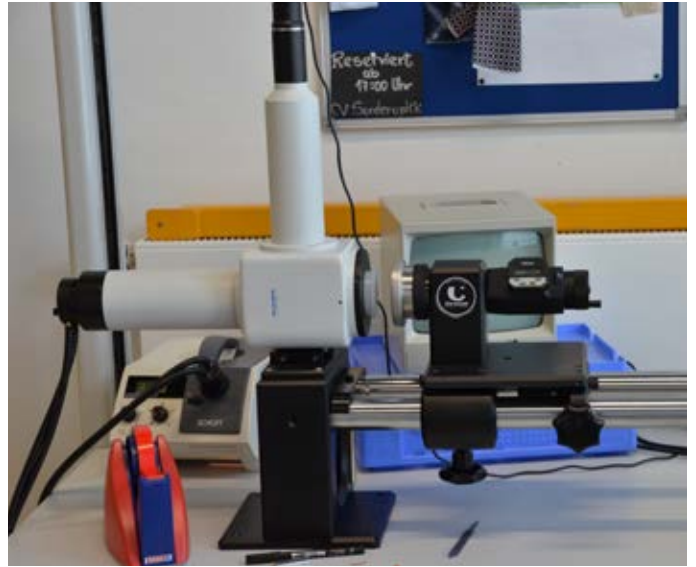
Leica uses some of the same test equipment familiar to all rental houses: here, a Chrosziel collimator.
