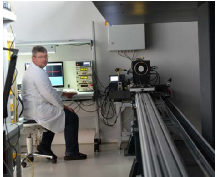
Now it gets really interesting: a very high-tech focus-scale indexing system on a 60' long "railroad" moves an MTF target to each marked distance to be engraved on the focus barrel.
